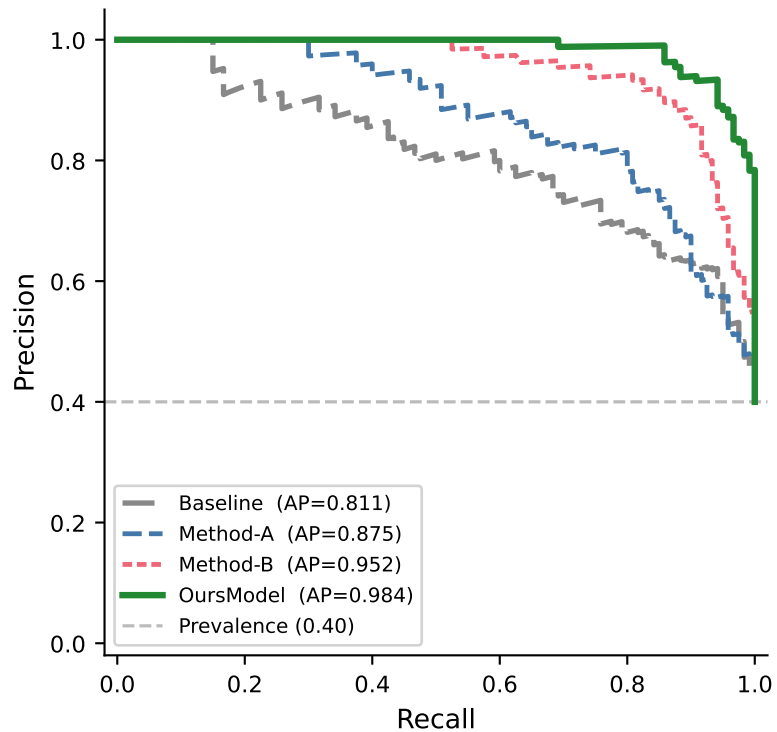
Precision-Recall Curve
