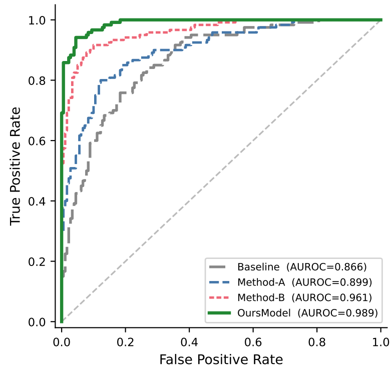
ROC Curve
