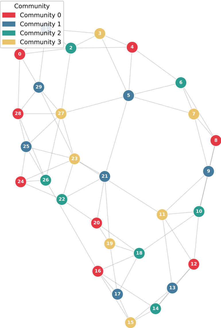
Force-directed network graph (30 nodes, 4 communities)
