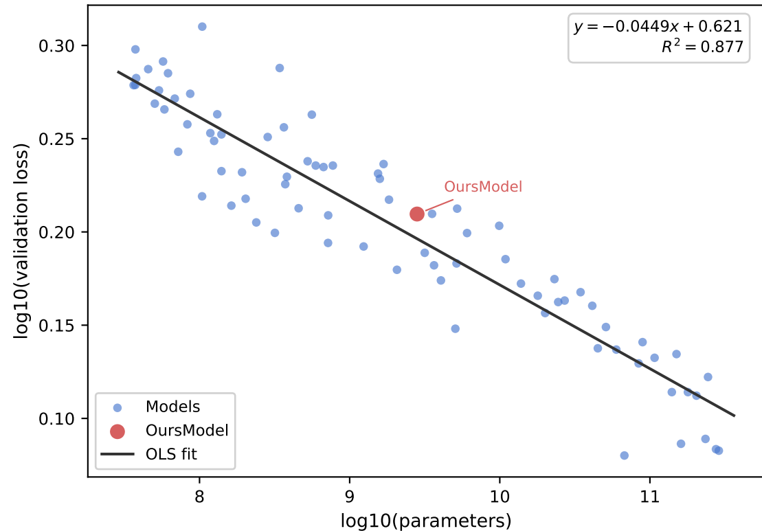
Scaling Law: Validation Loss vs. Model Size
