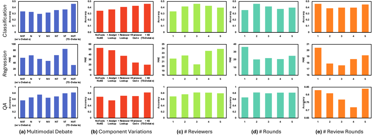
Figure 3: Impact of (a) modality composition, (b) system components, and (c–e) debate configurations across tasks.
