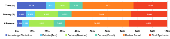
Figure 4: Average time and monetary cost breakdown.
