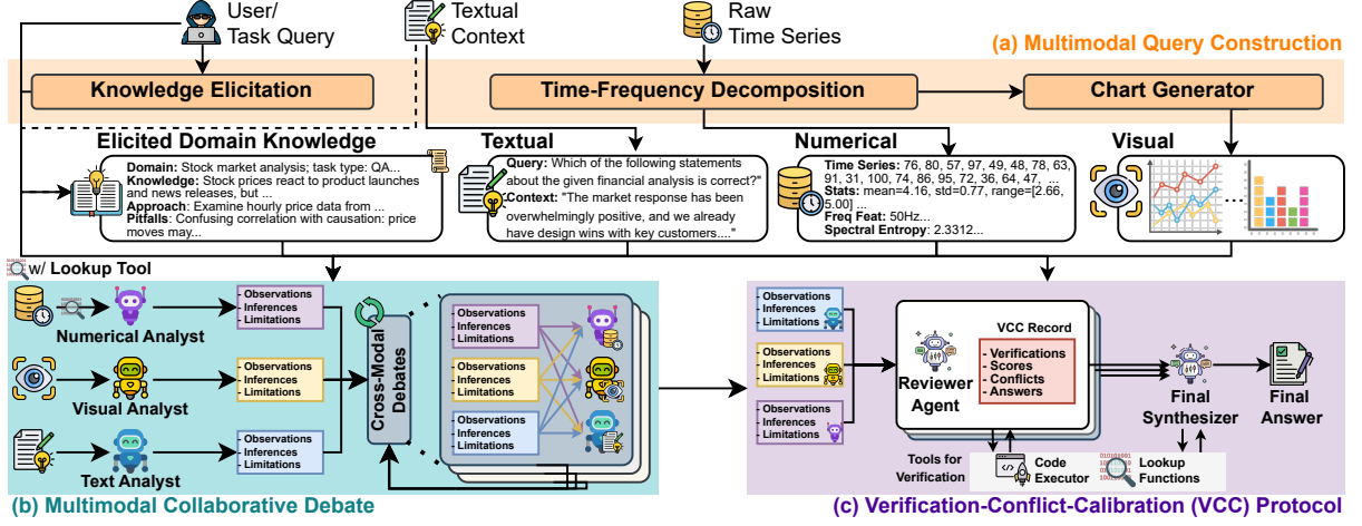
Figure 2: Overview of the TS-Debate framework. (a) Multimodal query construction derives textual, numerical, and visual representations from user queries, raw time series, and contextual information. (b) Multimodal collaborative debate enables numerical, visual, and text analysts to reason over these representations and produce structured observations, inferences, and limitations. (c) VCC protocol applies tool-assisted review to assess debate outputs, identify conflicts, and synthesize the final answer.
