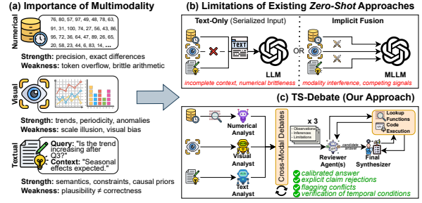
Figure 1: Overview of multimodal time-series reasoning: (a) complementary strengths and failure modes across modalities; (b) limitations of existing zero-shot approaches; and (c) TS-Debate, a cross-modal agentic framework with explicit verification.
