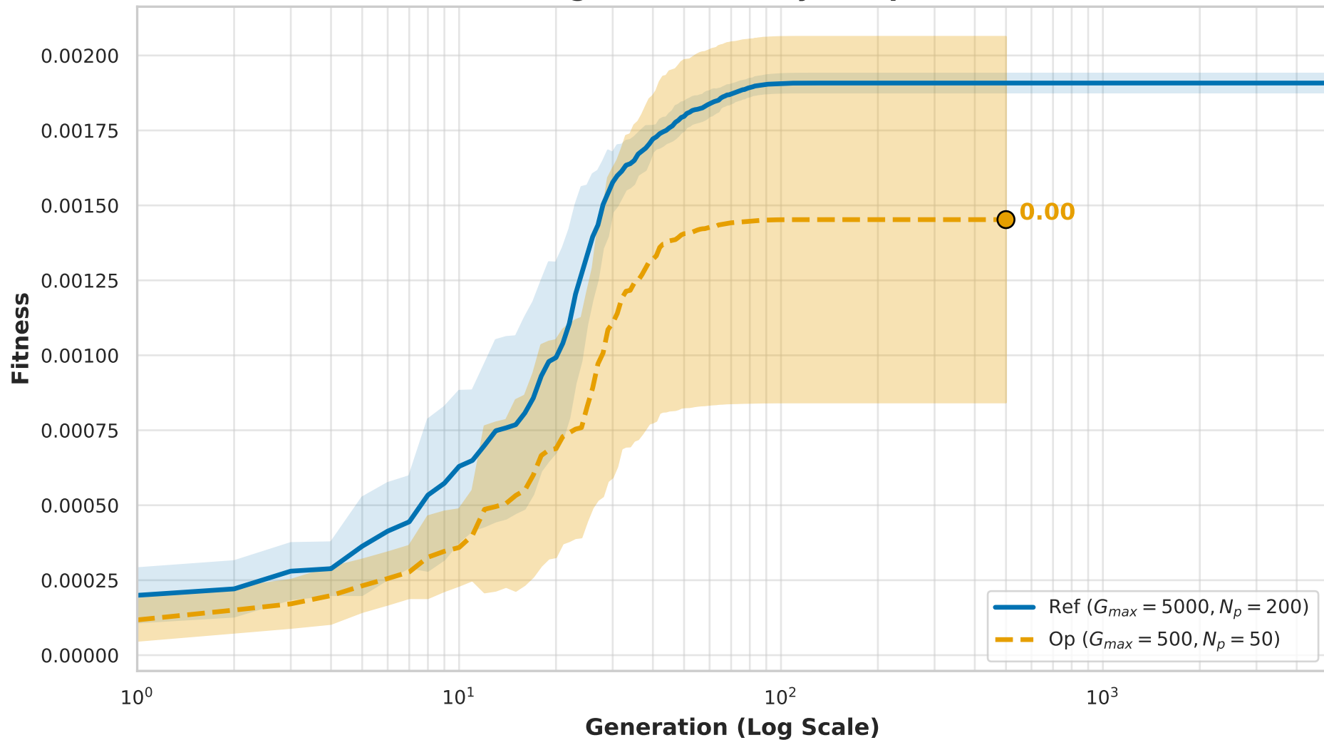
Convergence Efficiency Comparison
