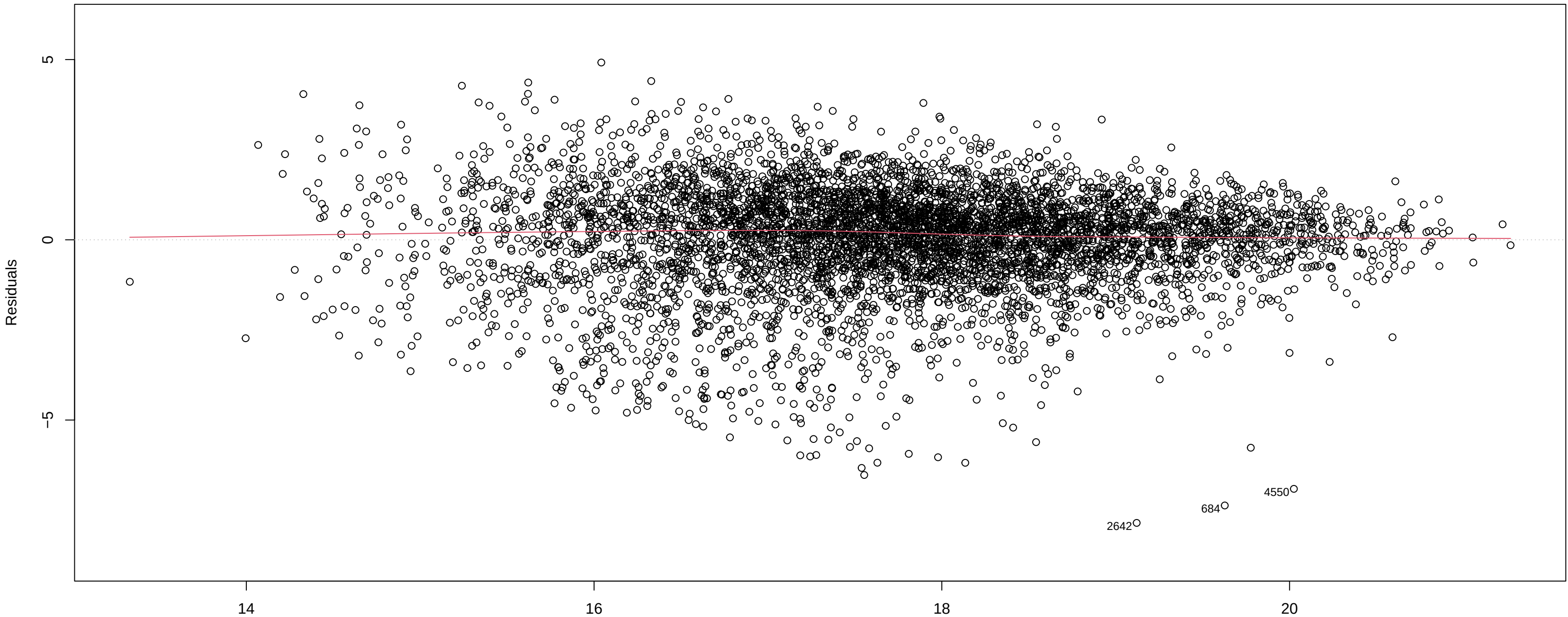
Residuals vs Fitted
