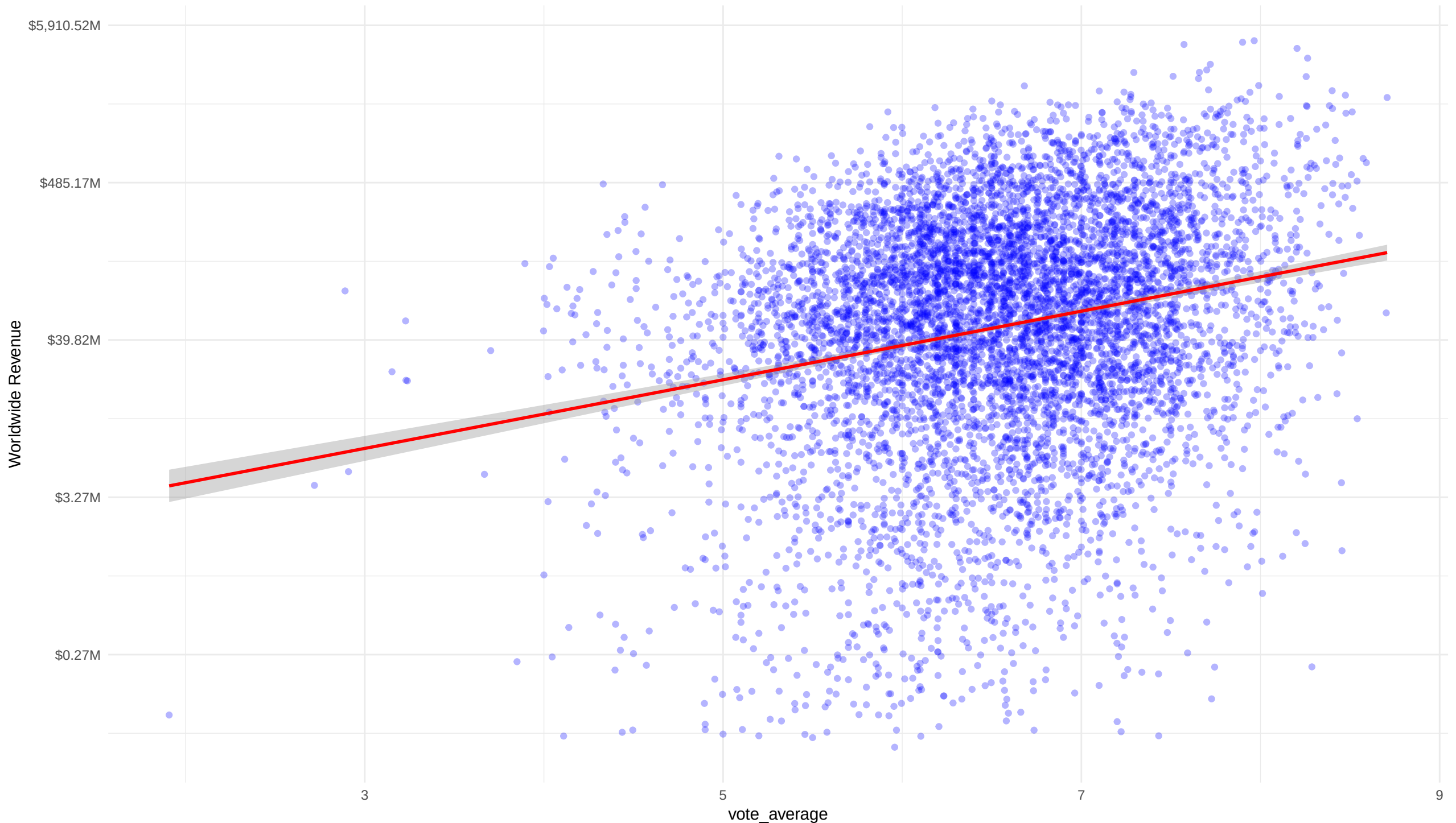
Movie vote avergae (out of 10) vs. Worldwide Revenue (ADJ for inflation) Based on Cleaned Data, Linear Model, R= 0.23 Weak Correlation
