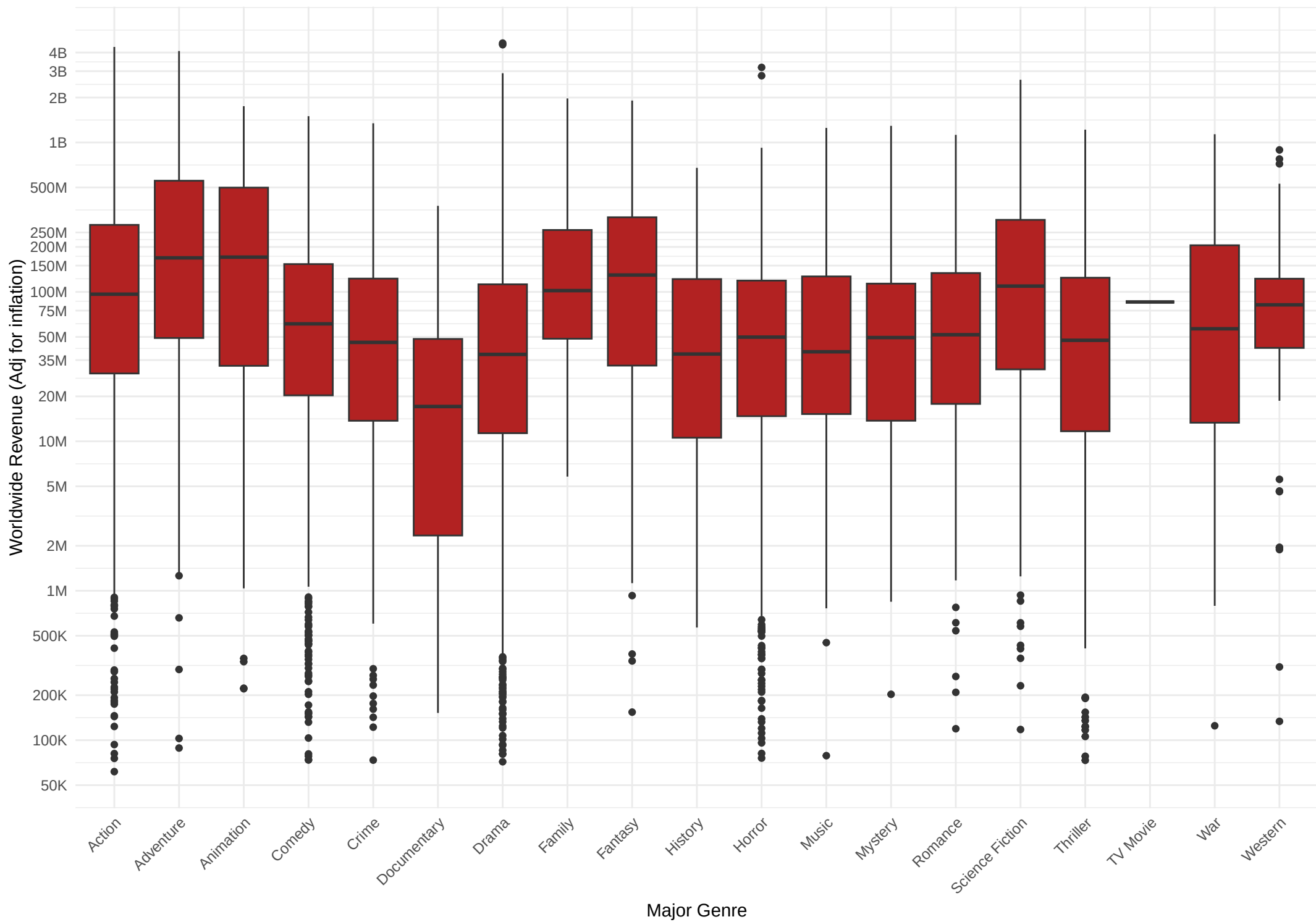
Boxplot of Genre Vs Worldwide Revenue
