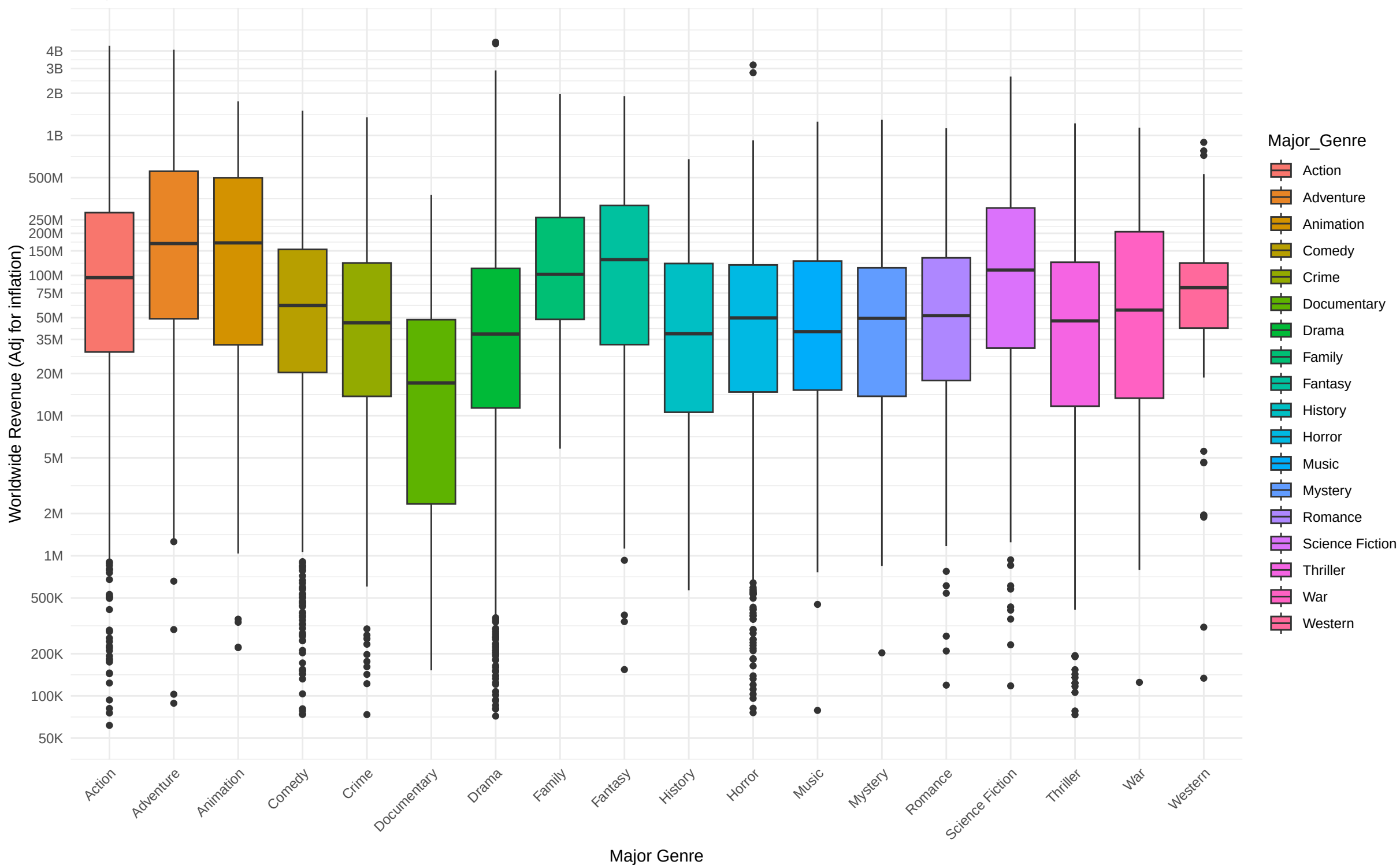
Boxplot of Genre Vs Worldwide Revenue
