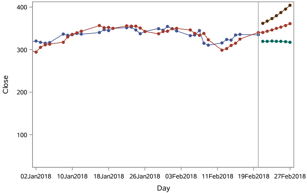
Plot of Forecasts for Tesla Close Price
