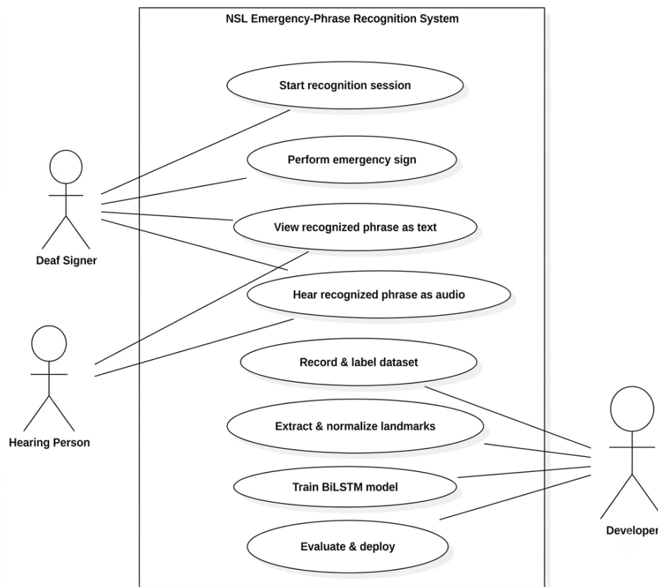
Figure 4.1: Use case diagram of the NSL emergency-phase recognition system
