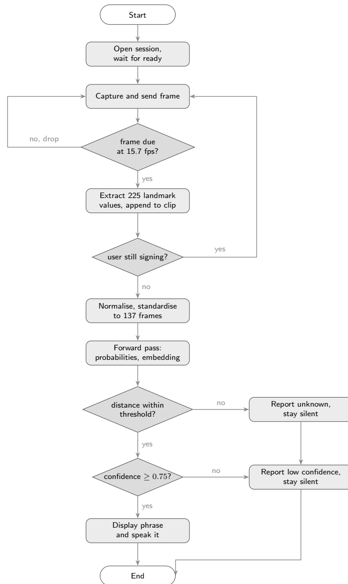
Figure 4.7: Activity diagram for one recognition attempt
