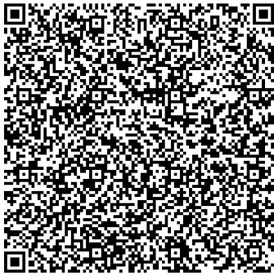
SEGMENT 18
