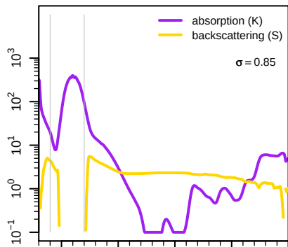
II. K-M Coefficient ( \text{mm}^{-1} )
