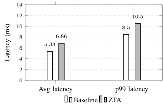
Fig. 3. Latency overhead introduced by ZTA policies (Fortio, 200 req, single connection). Baseline avg 5.33 ms, ZTA avg 6.86 ms; QPS drop: 187.5 → 145.7 (−22.3%).
