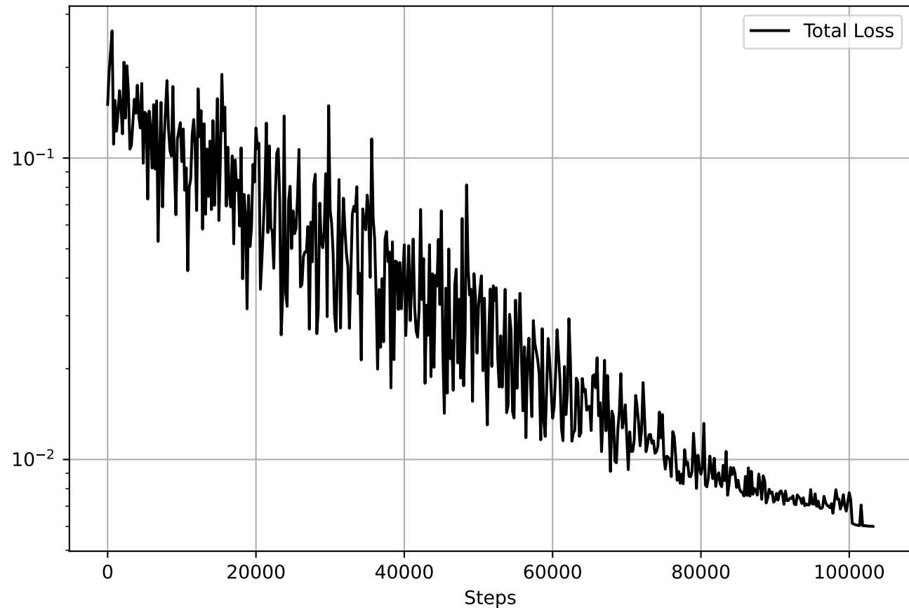
Phase 2 (Multi-mode): Total Loss
