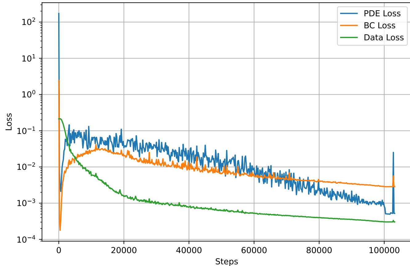
Phase 2 partial losses
