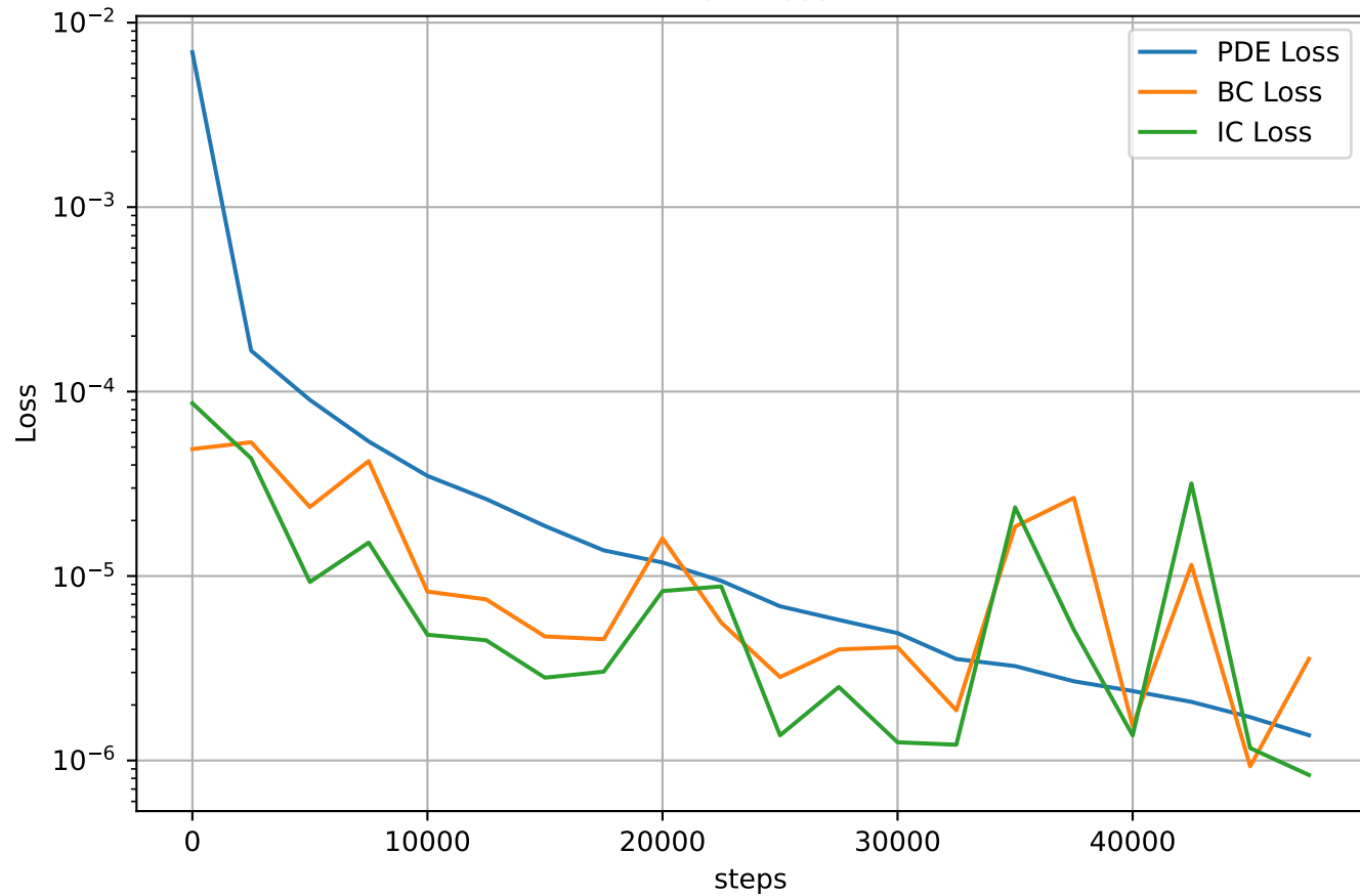
Train Loss
