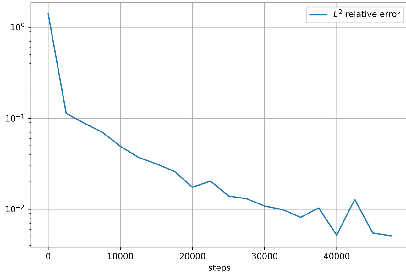
Test Loss
