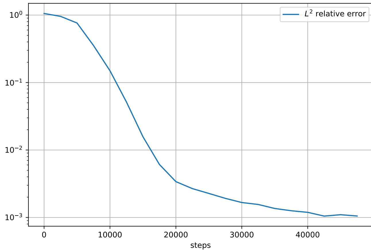
Test Loss
