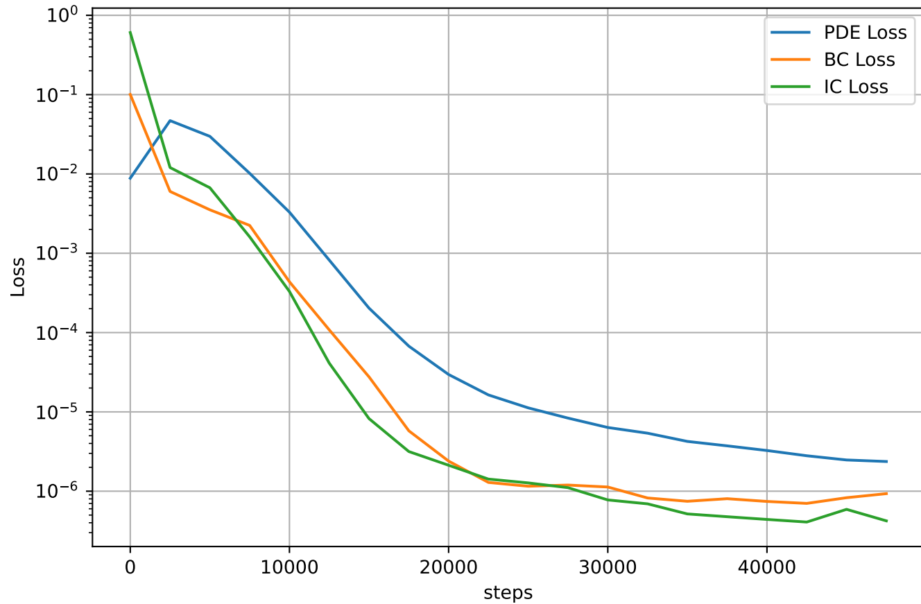
Train Loss
