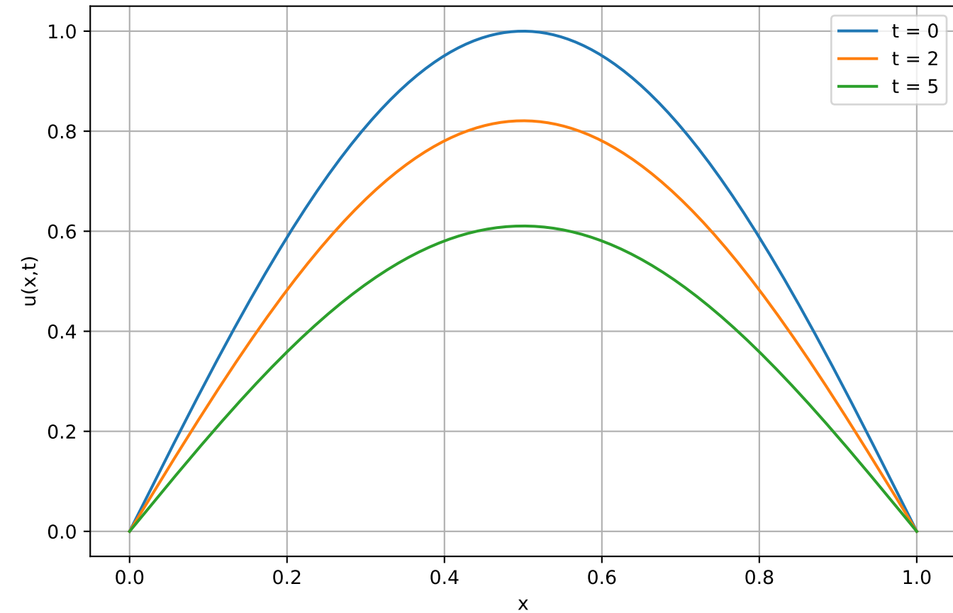
Exact Solution
