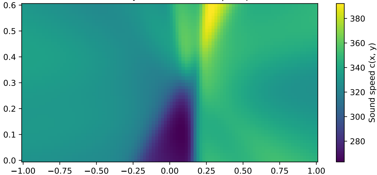
Reconstructed c(x,y) — Modes [0, 1] | Freqs [600] Hz
