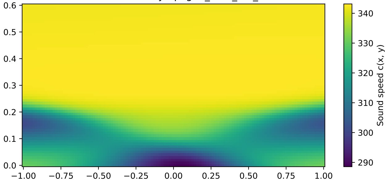
Inverted celerity - pkg01_f500_m0_1
