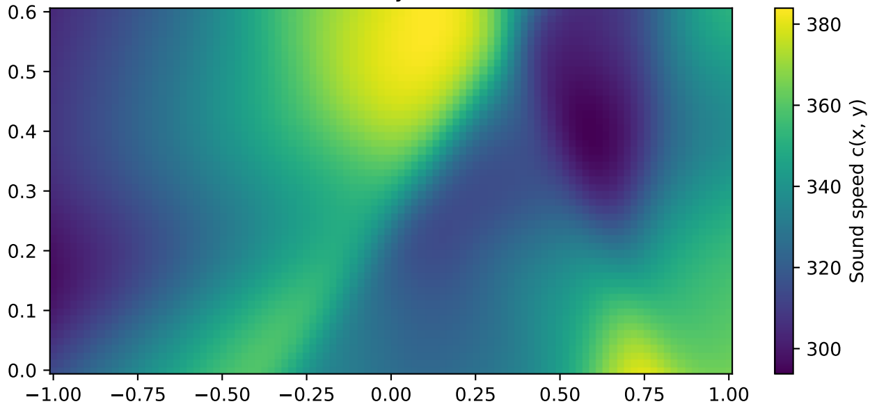
Reconstructed c(x,y) — 1000Hz:M[2]
