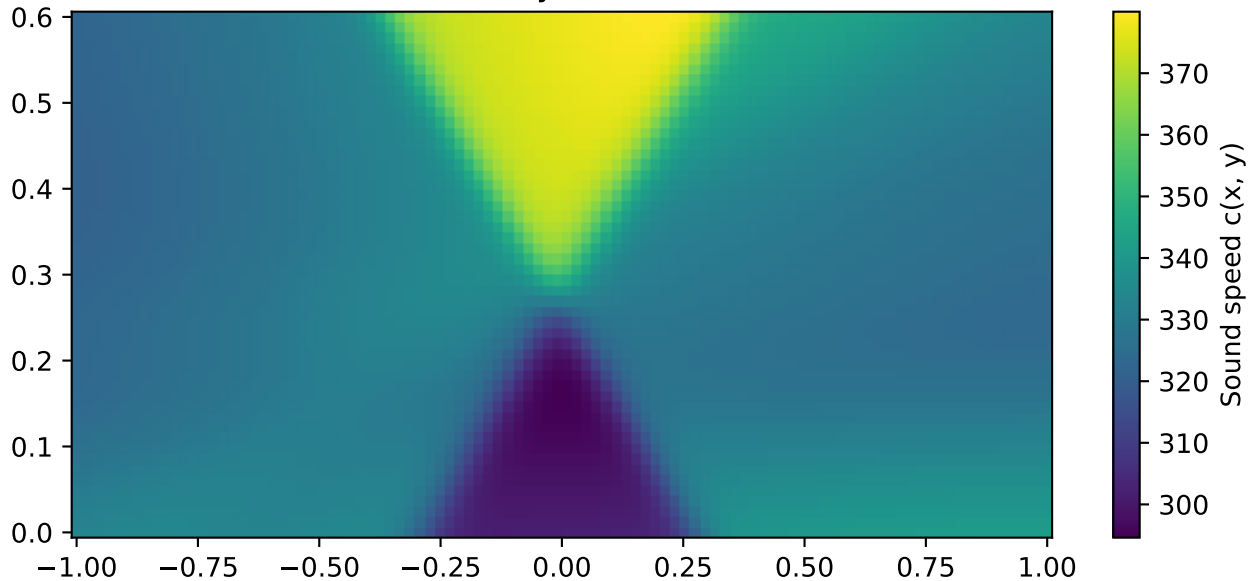
Reconstructed c(x,y) — 600Hz:M[0, 1, 2]
