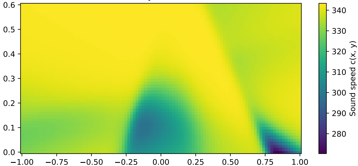
Reconstructed c(x,y) — 900Hz:M[0, 1, 2, 3]
