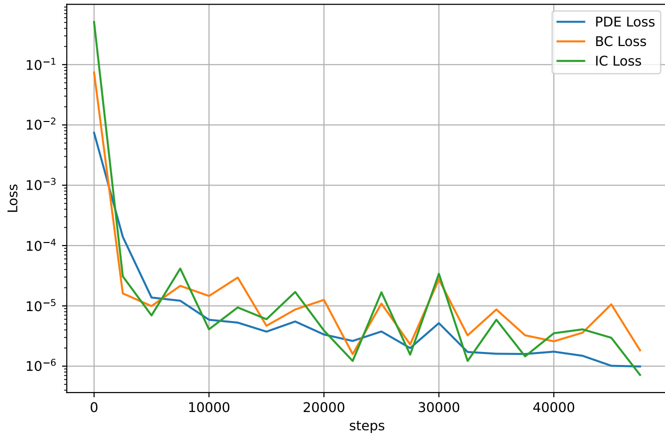
Train Loss
