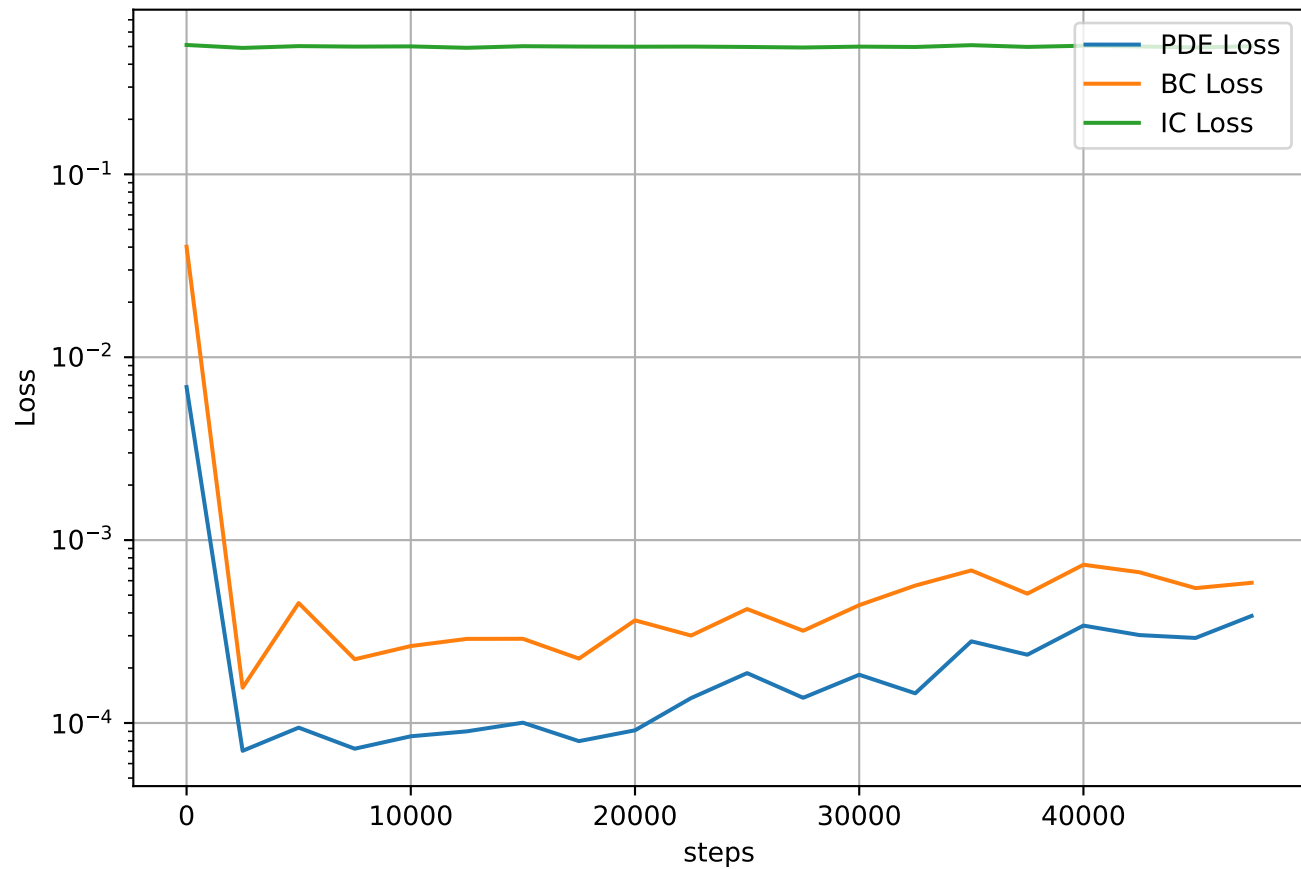
Train Loss
