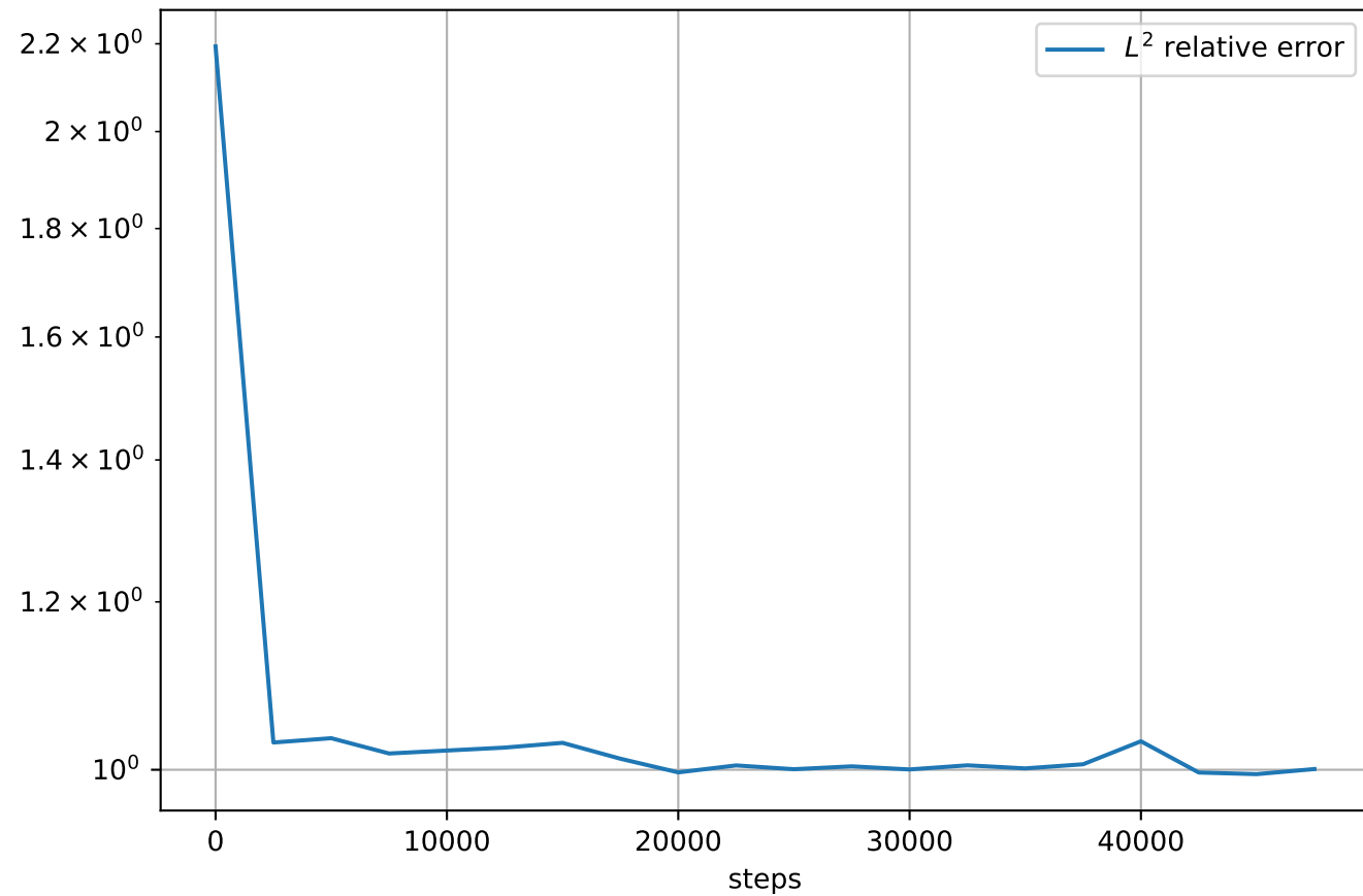
Test Loss
