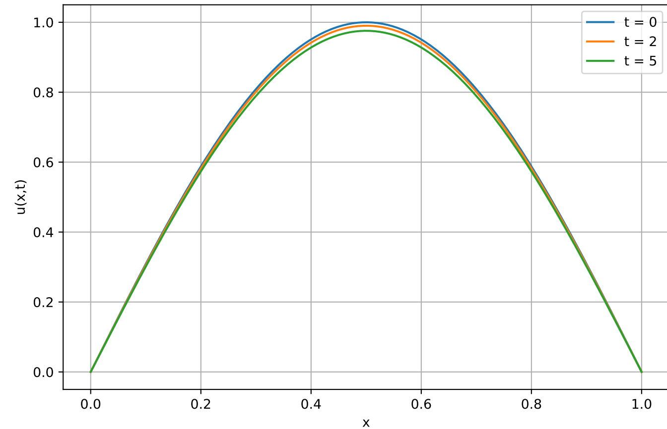
Exact Solution
