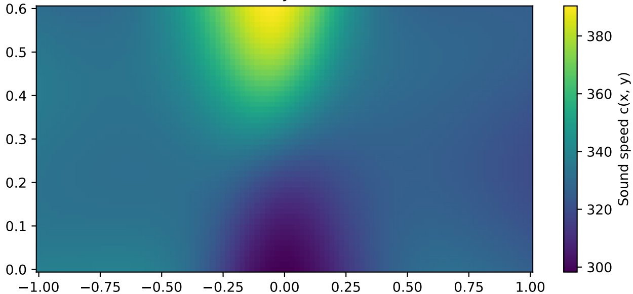
Reconstructed c(x,y) — 600Hz:M[0, 1]
