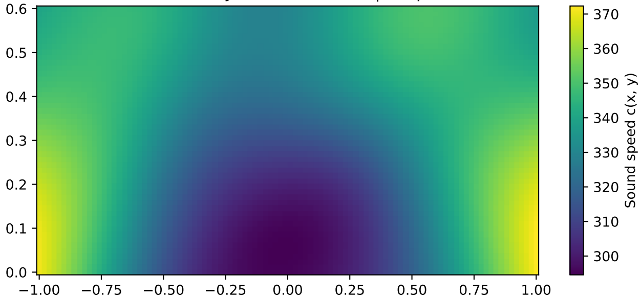
Reconstructed c(x,y) — Modes [0, 1] | Freqs [400] Hz
