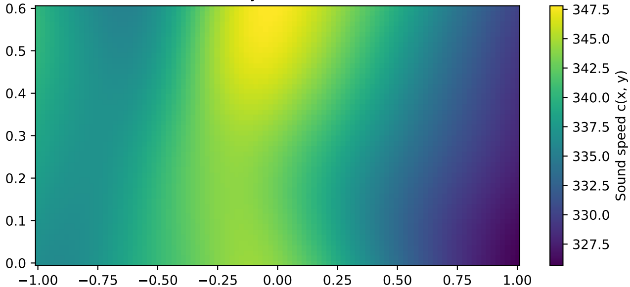
Reconstructed c(x,y) — 1500Hz:M[0, 1, 2, 3]
