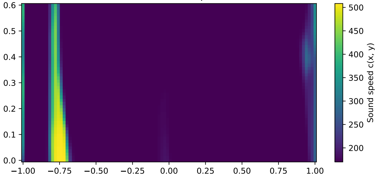
Reconstructed Sound Speed Field
