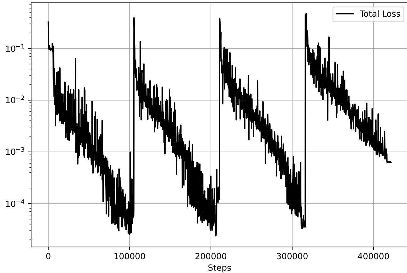
Phase 2: Total Loss
