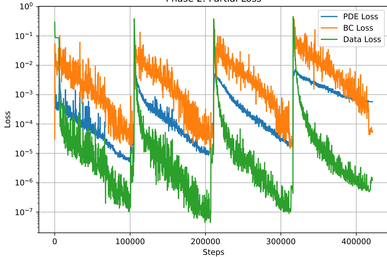
Phase 2: Partial Loss
