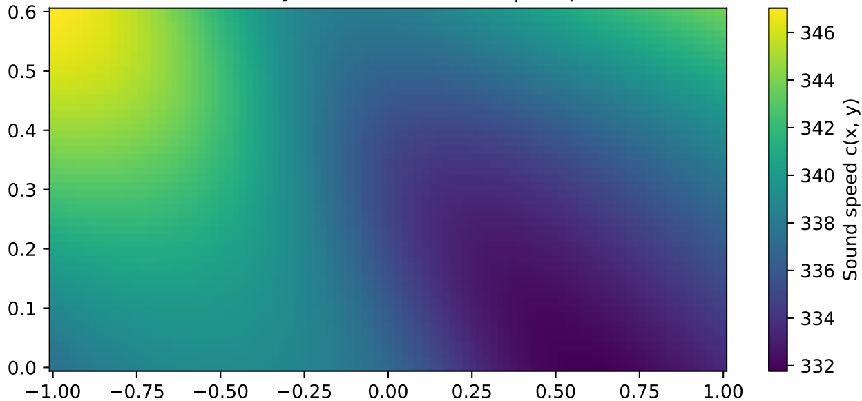
Reconstructed c(x,y) — Modes [0, 1, 2] | Freqs [1400] Hz
