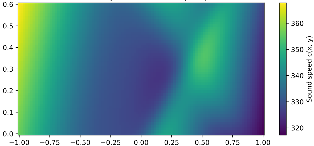
Reconstructed c(x,y) — Modes [1, 2] | Freqs [600] Hz
