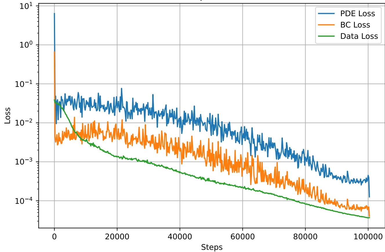
Inverse partial losses
