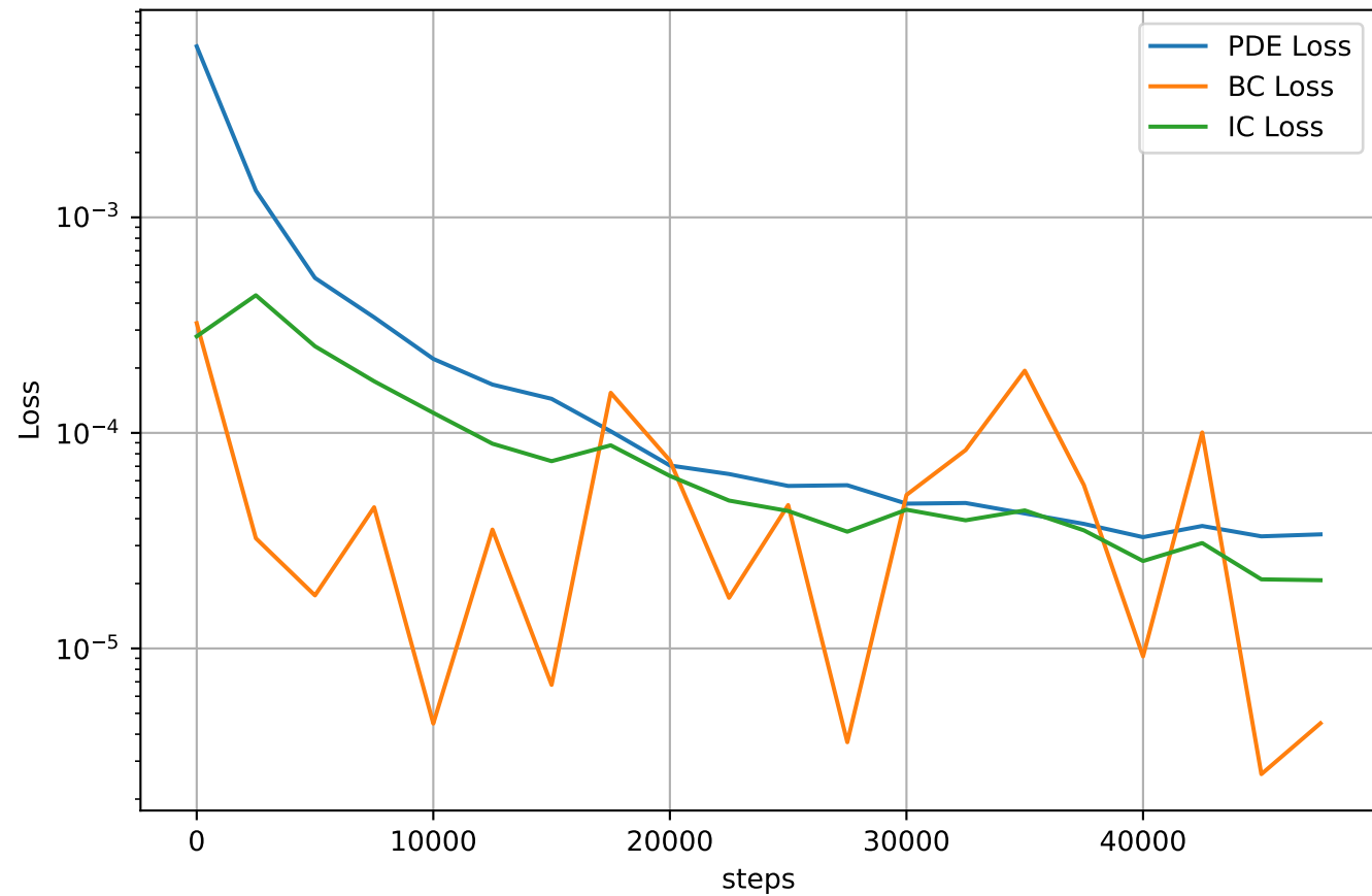
Train Loss
