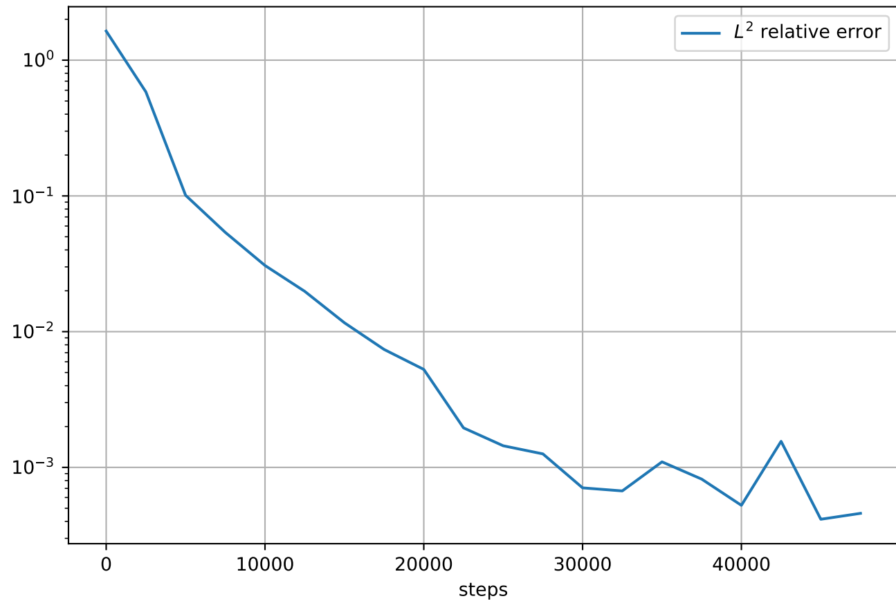
Test Loss
