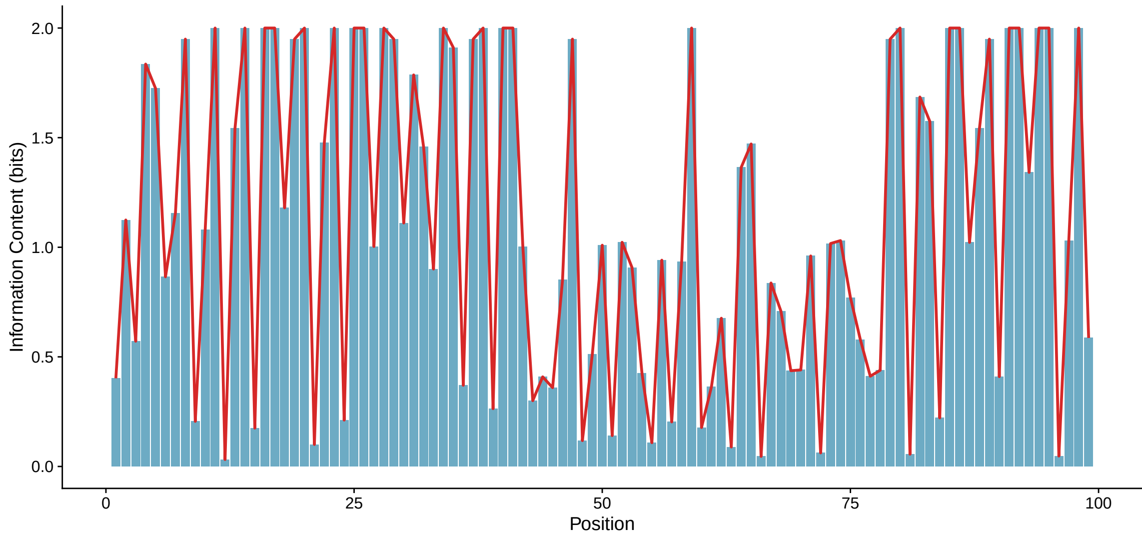
Nucleotide Conservation Across and Around Motif
