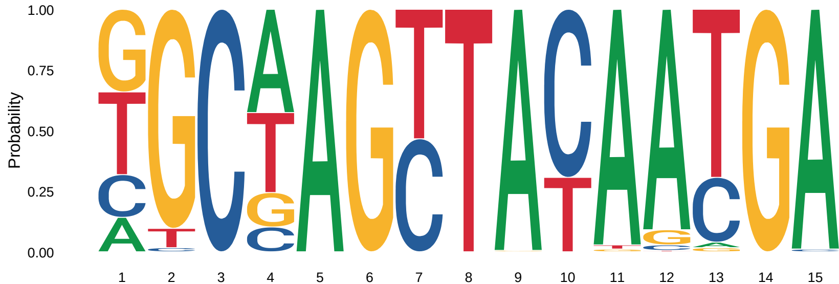
Observed catalytic-core windows vs canonical GGCTAGCTACAACGA
