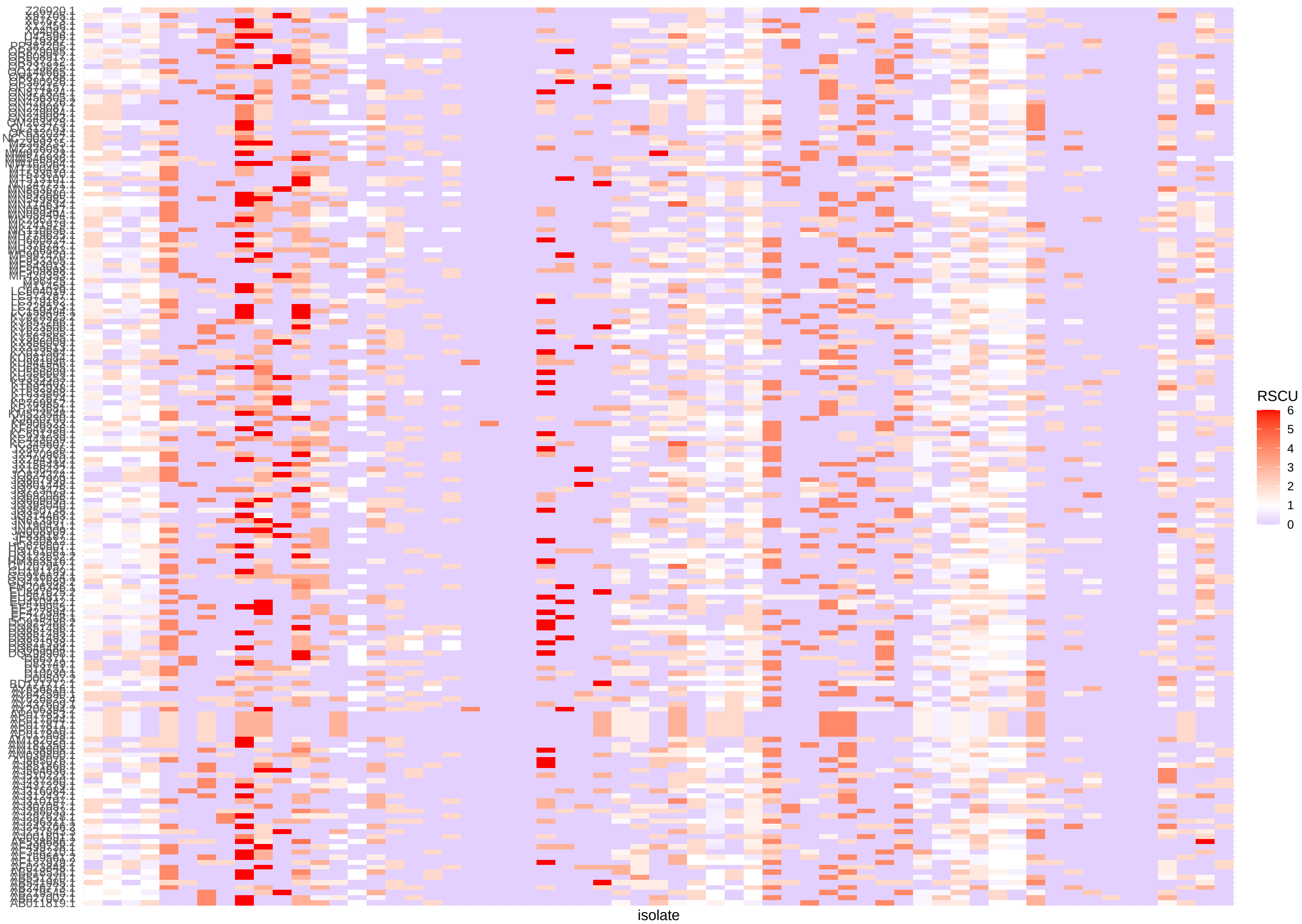
RSCU Heatmap — Motif Sequences
