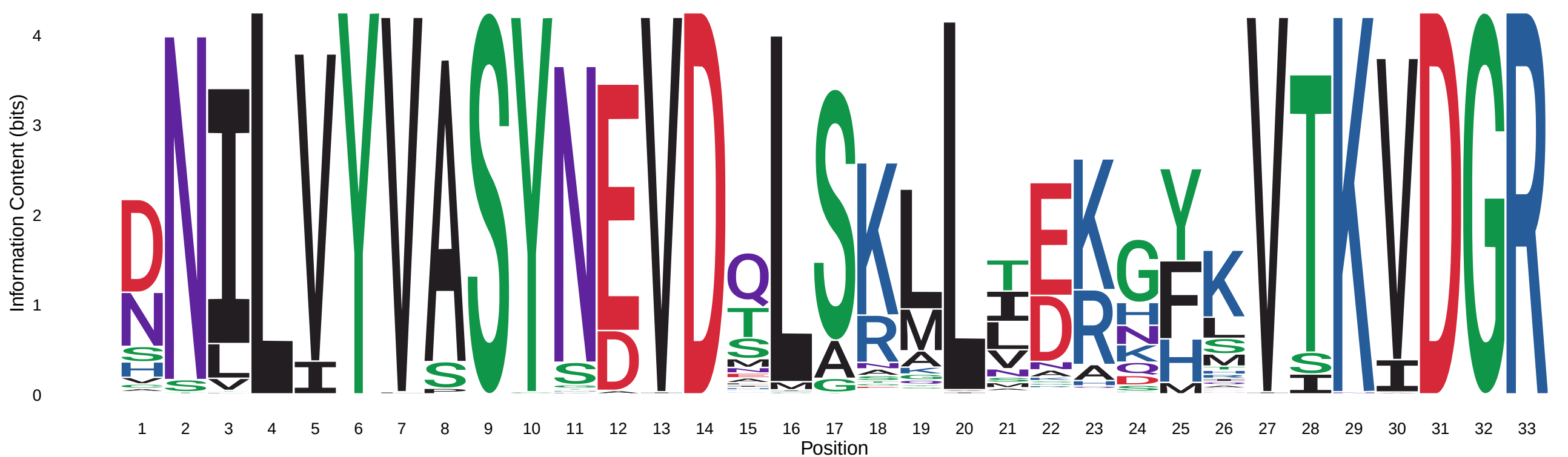
18nt Motif – Protein Sequence Logo
