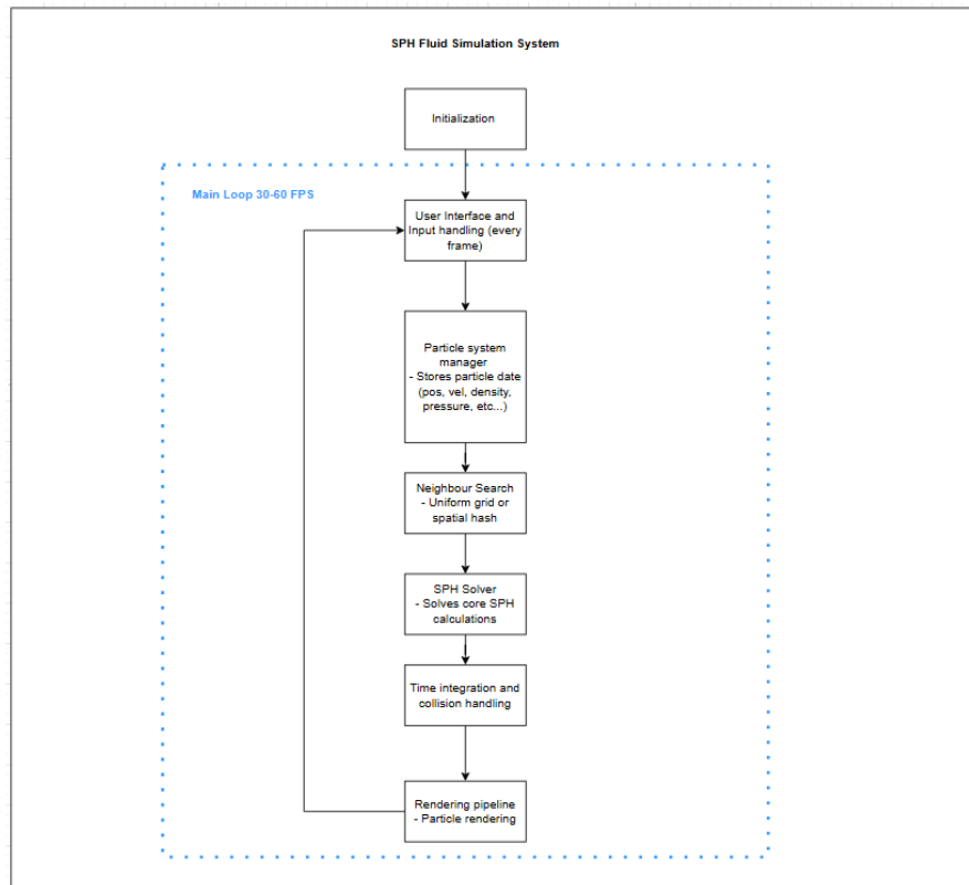
Figure 1: SPH Fluid Simulation System Architecture Diagram
