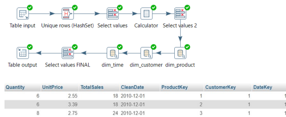
Fig. 4. Fact Sales transformation workflow and output table.
