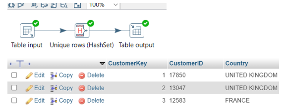
Fig. 2. Customer dimension transformation workflow and output table.
