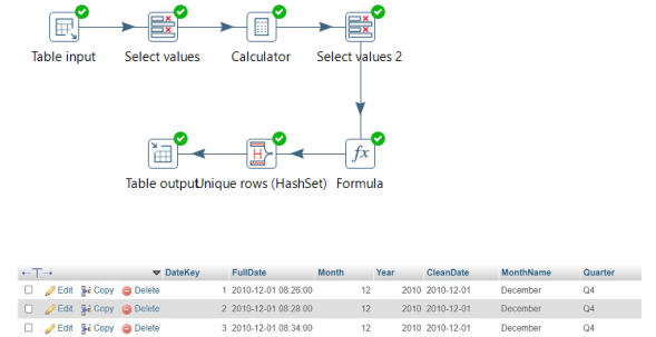
Fig. 3. Time dimension transformation workflow and output table.
