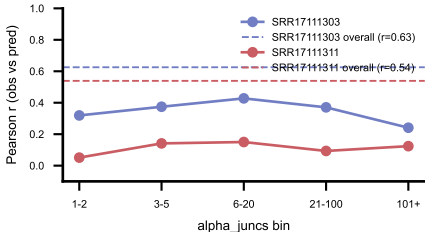
SSU prediction quality vs depth (dashed = overall across all bins)
