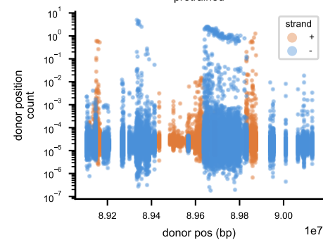
pretrained
