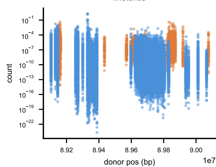
finetuned
