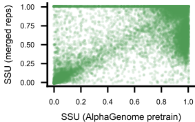
ssu_approx ( \alpha/\alpha+\beta_2 ) r=0.818 n=29,773
