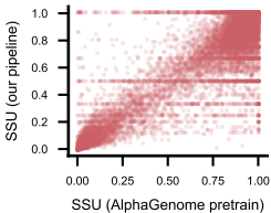
K562 rep2 r = 0.942 n = 27,593
