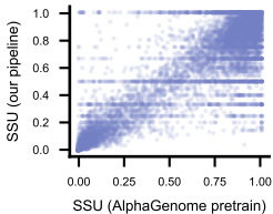
K562 rep1 r = 0.934 n = 25,808
