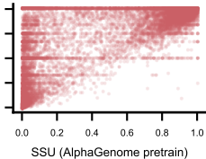
ssu_b1only ( \alpha/\alpha+\beta_1 ) r=0.736 n=29,681
