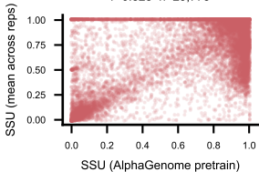
ssu_approx ( \alpha/\alpha+\beta_2 ) r=0.828 n=29,773
