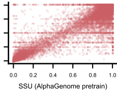
ssu_spliser ( \alpha/\alpha+\beta_1+\beta_2 ) r=0.947 n=29,681
