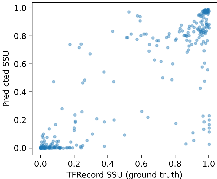
K562 polyA+ SSU TFRecord vs model prediction r = 0.852
