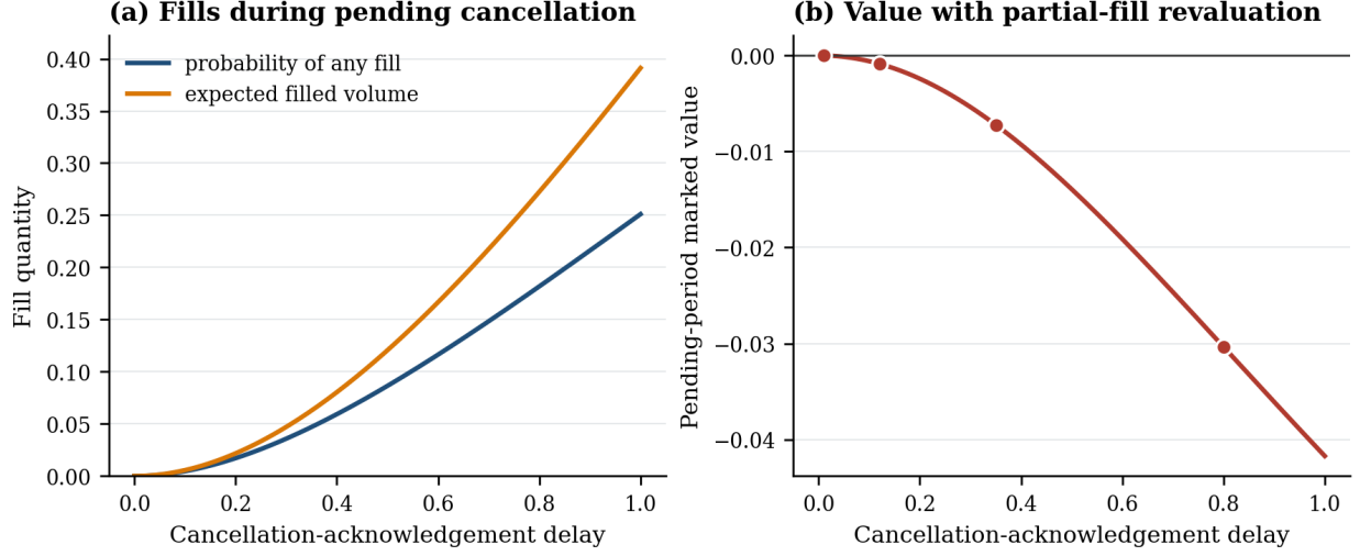
Figure 4: A still-live order during cancellation latency. Starting with three lots ahead and two tagged lots, panel (a) evaluates the compound Poisson law for the probability of any fill and expected filled volume. Panel (b) evaluates the exact pending-period value V^d , including the revaluation of earlier partial fills and post-acknowledgement inventory. The markers are the four delays reported in the table. All quantities come from the declared nine-state synthetic queue cell.
