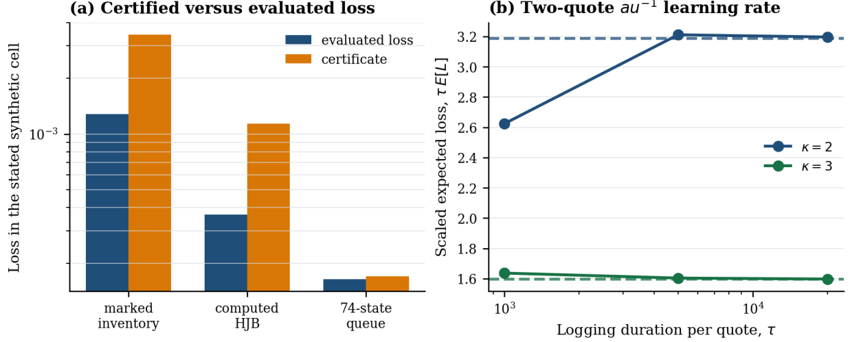
Figure 3: Certificates and learning rates in separate synthetic cells. Panel (a) compares independently evaluated policy loss with its applicable certificate for the marked-inventory model, the computed HJB model, and the 74-state queue model; the logarithmic scale is shared, but each pair retains its own declared model units. Panel (b) shows exact Poisson-sum evaluations of \tau \mathbb{E}[L] for \kappa = 2, 3 , converging to the constants in (40) (dashed lines). No simulated sampling or market data are used.
