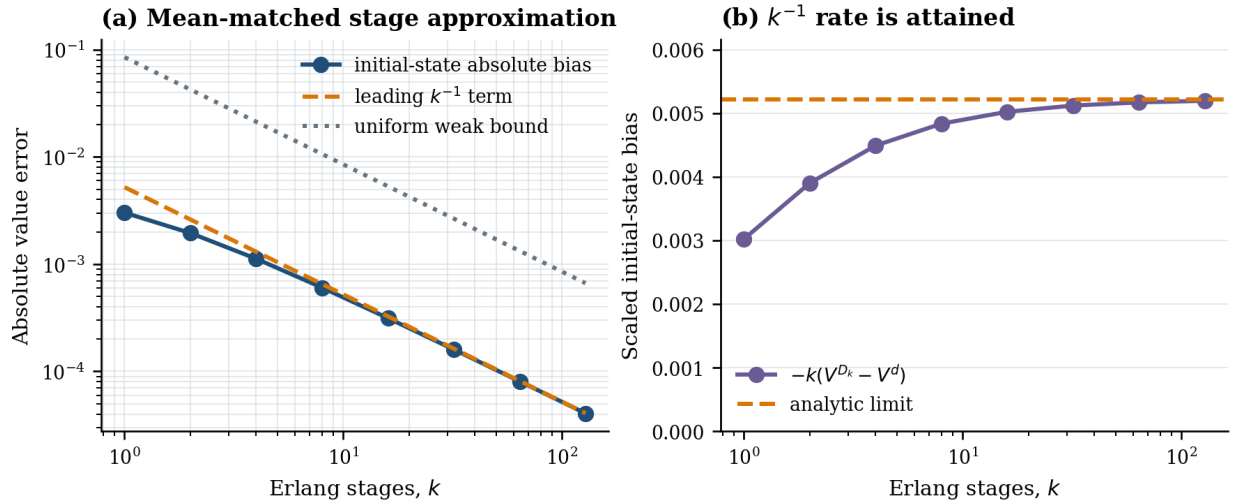
Figure 5: Mean-matched Erlang approximation of deterministic cancellation latency at d = 0.35 . Panel (a) compares the initial-state absolute bias with the leading k^{-1} term and the uniform weak bound from Theorem 3.11. Panel (b) shows that -k(V^{D_k} - V^d) approaches the analytic coefficient 0.00521944. The independent stage recursion and matrix calculation use the same nine-state synthetic cell as Figure 4.
