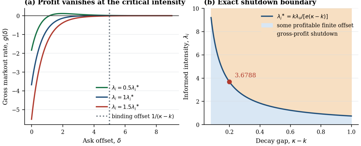
Figure 2: Exact gross-profit shutdown geometry. Panel (a) plots g(\delta) for \lambda_u = 2 , \kappa = 1.2 , k = 1 , and informed intensities equal to one half, exactly, and one and a half times the critical value. At equality the maximum is zero at \delta = 1/(\kappa - k) = 5 . Panel (b) plots \lambda_i^* = k\lambda_u/[e(\kappa - k)] ; the red point is the threshold 10/e from the arithmetic example. The shaded regions indicate whether some finite offset has positive gross markout under the stated static criterion.
