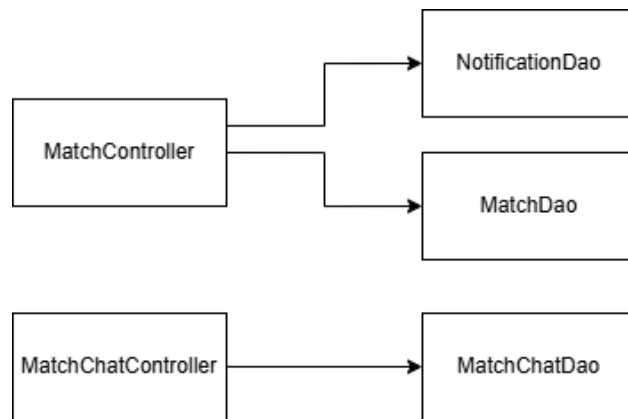
Figure 2: Iteration 3 - Live Matches Simplified Class Diagram
